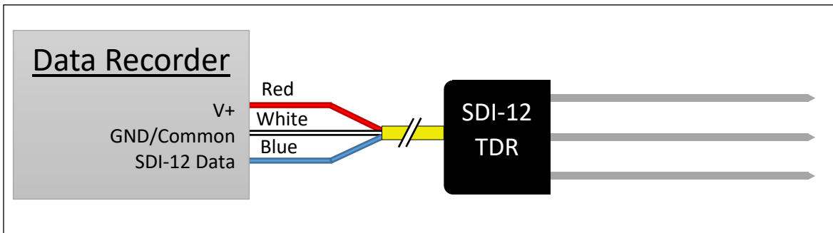
Figure 2: Connecting TDR Sensors to Data Recorder with Power Output
