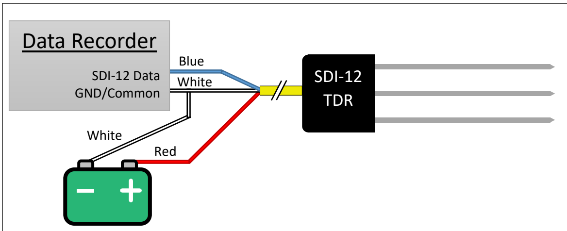
Figure 1: Connecting TDR sensors to a Data Recorder with a Separate Power Source for the Sensors
