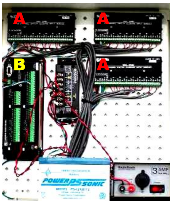
Figure 2-10. Control board detail, flowmeter-datalogger boxes showing A) multiplexers, B) CR 10X datalogger used for this study.
