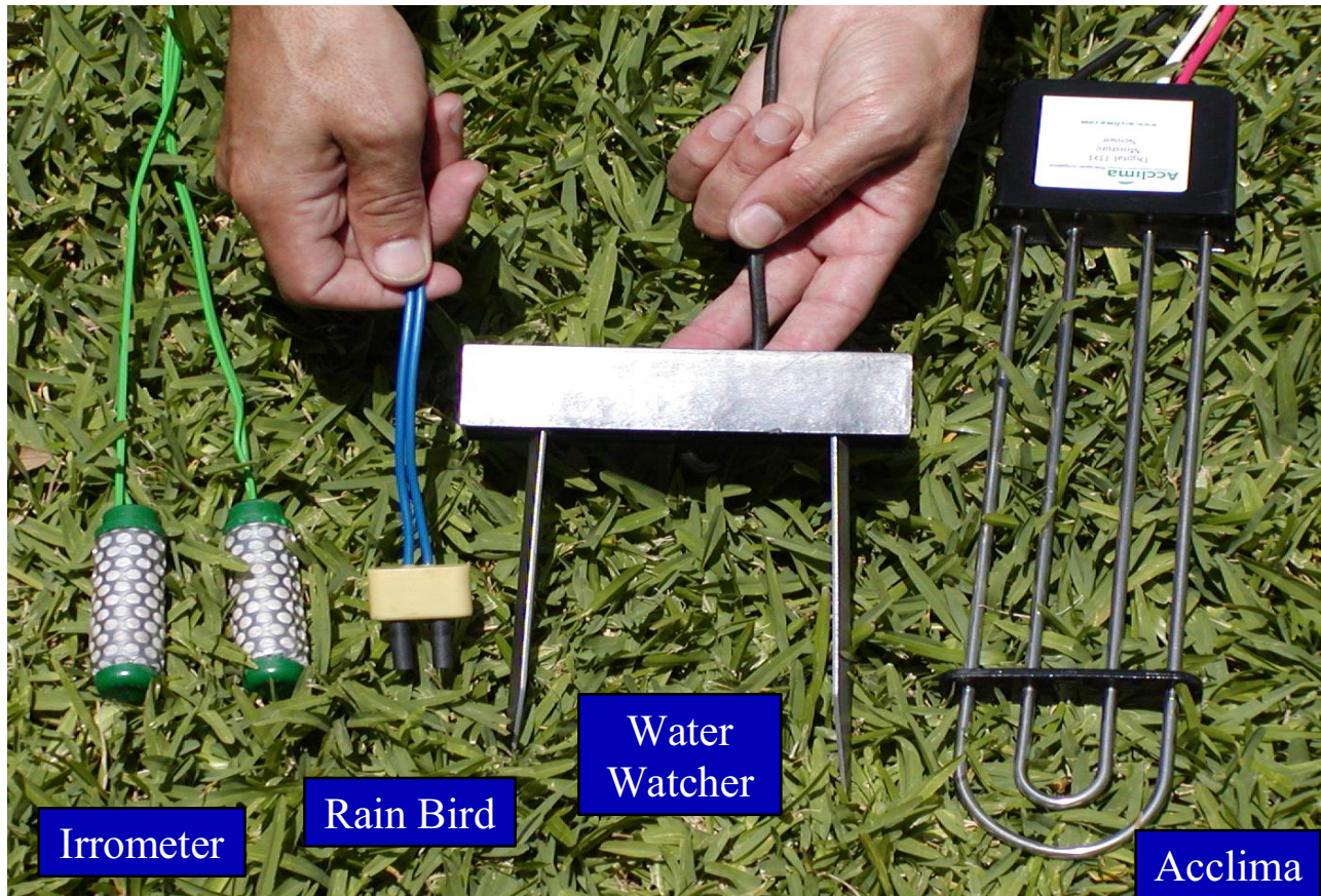
Figure 2-4. Sensors tested in the experiment: Irrometer, Rain Bird, Water Watcher and Acclima.
