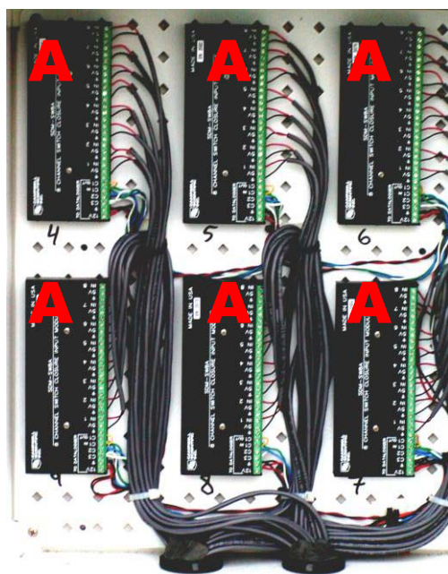
Figure 2-10. Control board detail, flowmeter-datalogger boxes showing A) multiplexers, B) CR 10X datalogger used for this study.
