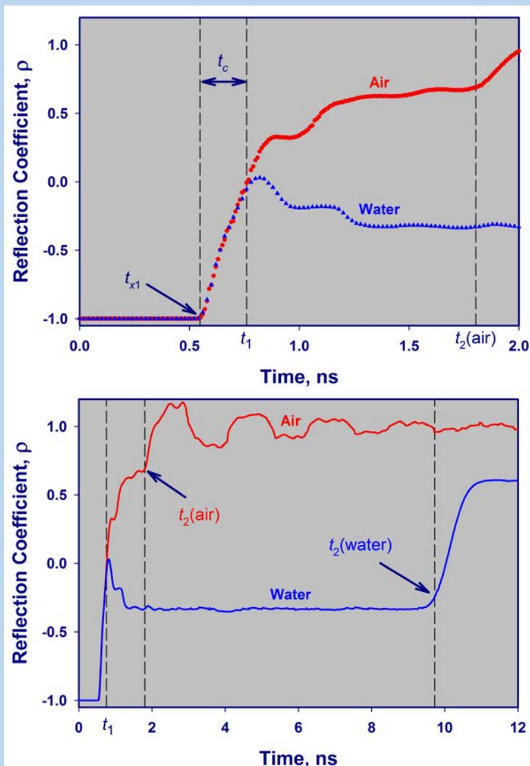
Fig. 2. Waveforms in air and deionized water acquired using a TDR-315 probe showing the time of the step signal launch ( t_{s1} ), time at which the signal enters the media ( t_1 ) and the time of the reflection at the end of the rod in air, t_2(\text{air}) , and water t_2(\text{water}) determined using AWIGF (Schwartz et al., 2014). The offset, t_c , is fitted based on the calibration in air and water.
