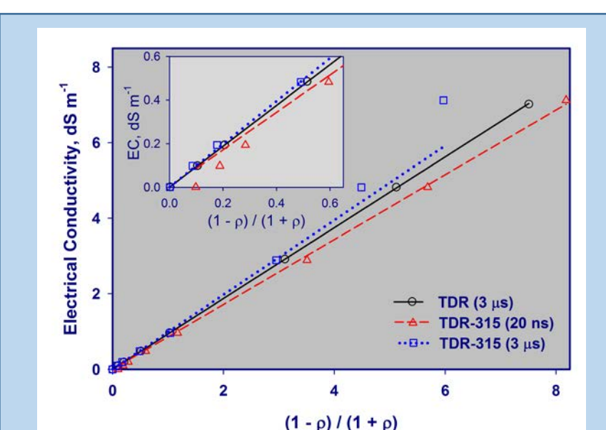
Fig. 3. Electrical conductivity (EC) calibrations for the long time reflection coefficient, \rho , in \text{CaCl}_2 solutions for the TDR and TDR-315. Inset shows calibration response at low EC levels.
